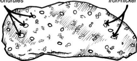
The polished face of a chondrite meteorite
