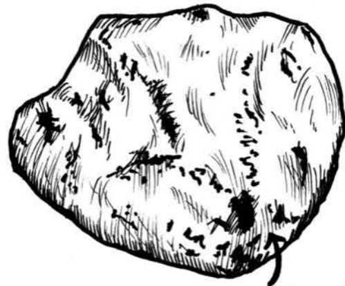
The fusion crust of a stony meteorite
