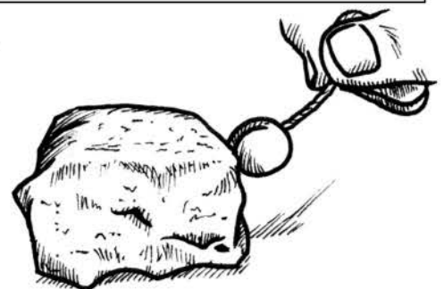
The magnet test – magnets are often strongly attracted to meteorites
